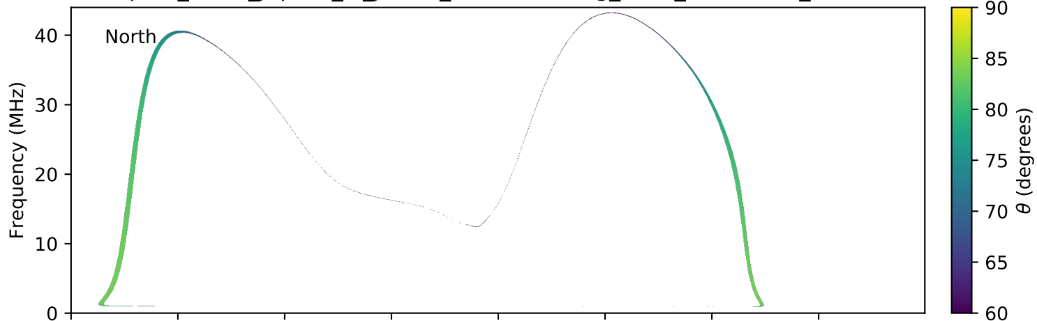
expres_earth_jupiter_io_jrm09_lossc-wid1deg_3kev_20100102_v01.cdf
