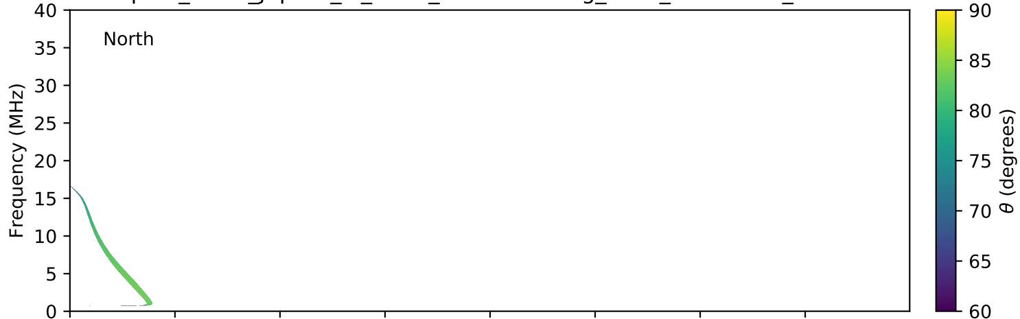
expres_earth_jupiter_io_isaac_lossc-wid1deg_3kev_20100131_v01.cdf
