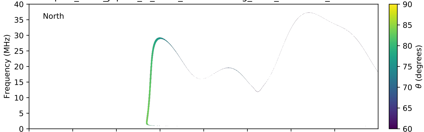
expres_earth_jupiter_io_isaac_lossc-wid1deg_3kev_20100130_v01.cdf
