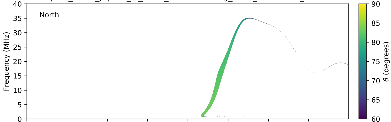
expres_earth_jupiter_io_isaac_lossc-wid1deg_3kev_20100128_v01.cdf
