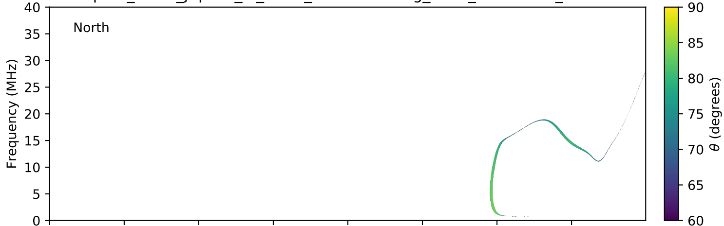
expres_earth_jupiter_io_isaac_lossc-wid1deg_3kev_20100126_v01.cdf
