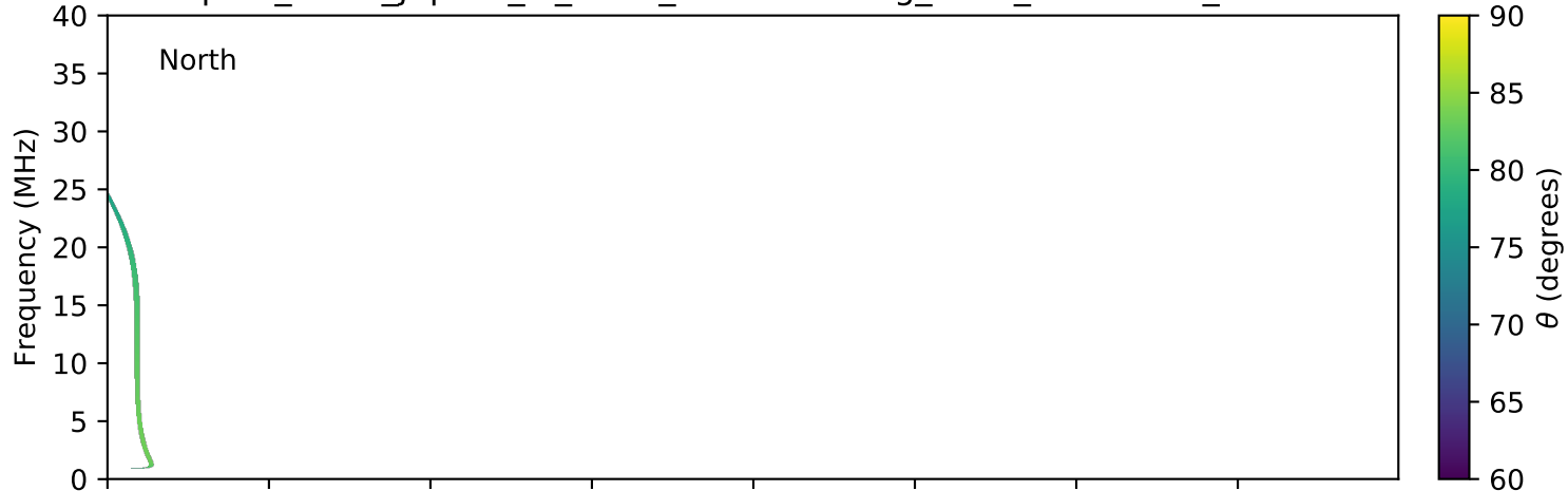
expres_earth_jupiter_io_isaac_lossc-wid1deg_3kev_20100124_v01.cdf
