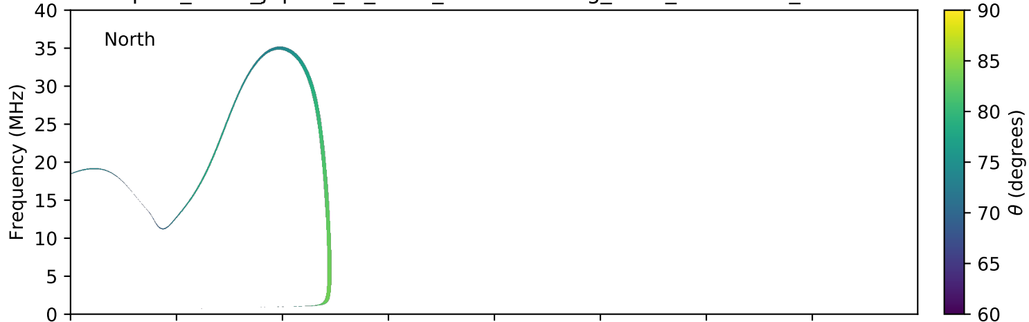
expres_earth_jupiter_io_isaac_lossc-wid1deg_3kev_20100122_v01.cdf
