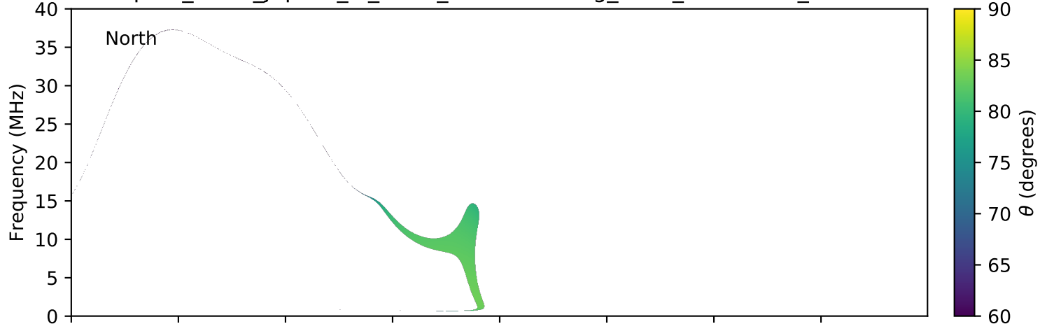
expres_earth_jupiter_io_isaac_lossc-wid1deg_3kev_20100120_v01.cdf
