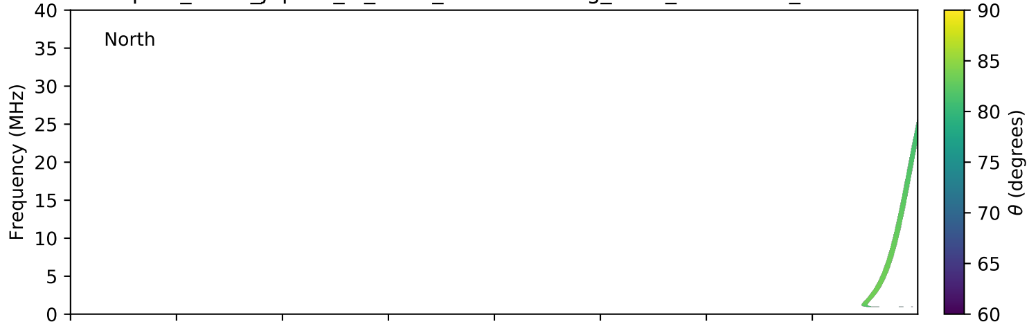
expres_earth_jupiter_io_isaac_lossc-wid1deg_3kev_20100117_v01.cdf
