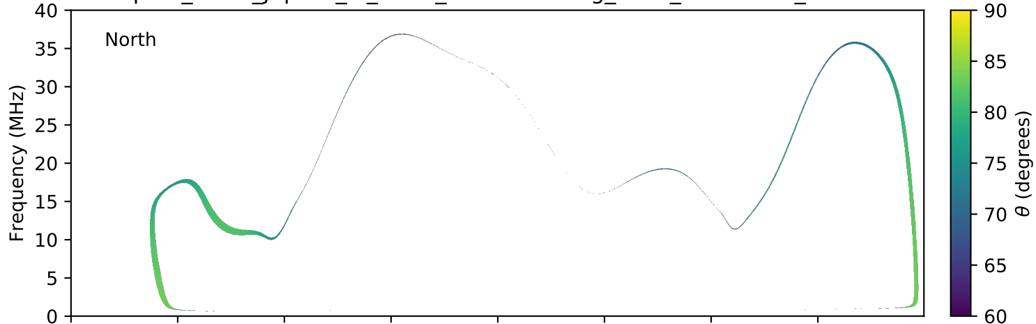
expres_earth_jupiter_io_isaac_lossc-wid1deg_3kev_20100116_v01.cdf
