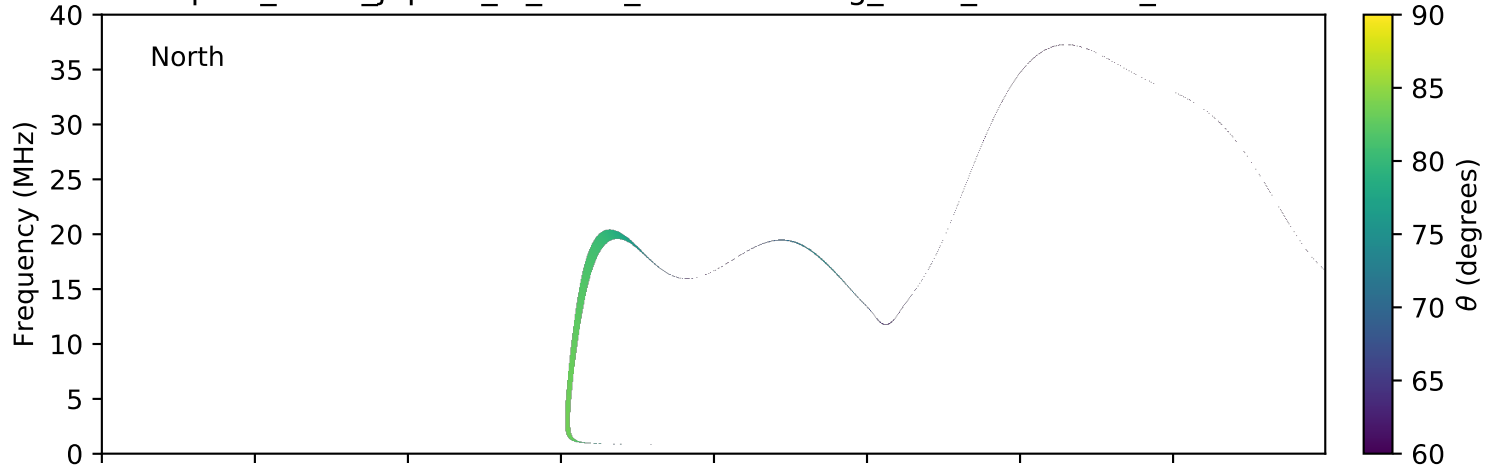
expres_earth_jupiter_io_isaac_lossc-wid1deg_3kev_20100114_v01.cdf
