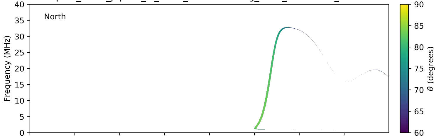
expres_earth_jupiter_io_isaac_lossc-wid1deg_3kev_20100112_v01.cdf
