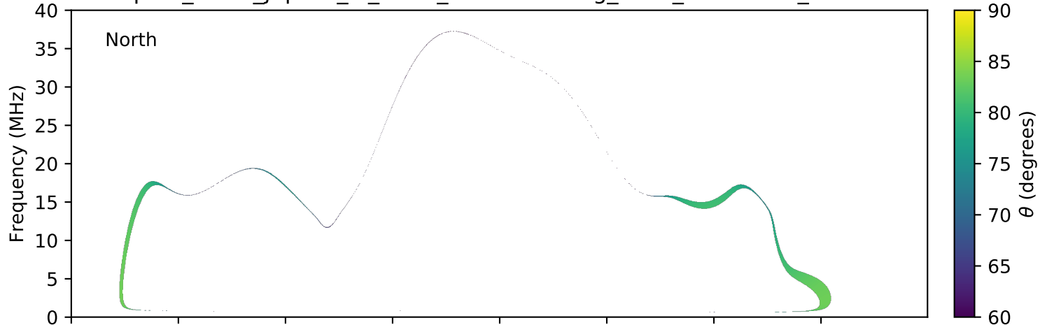
expres_earth_jupiter_io_isaac_lossc-wid1deg_3kev_20100109_v01.cdf
