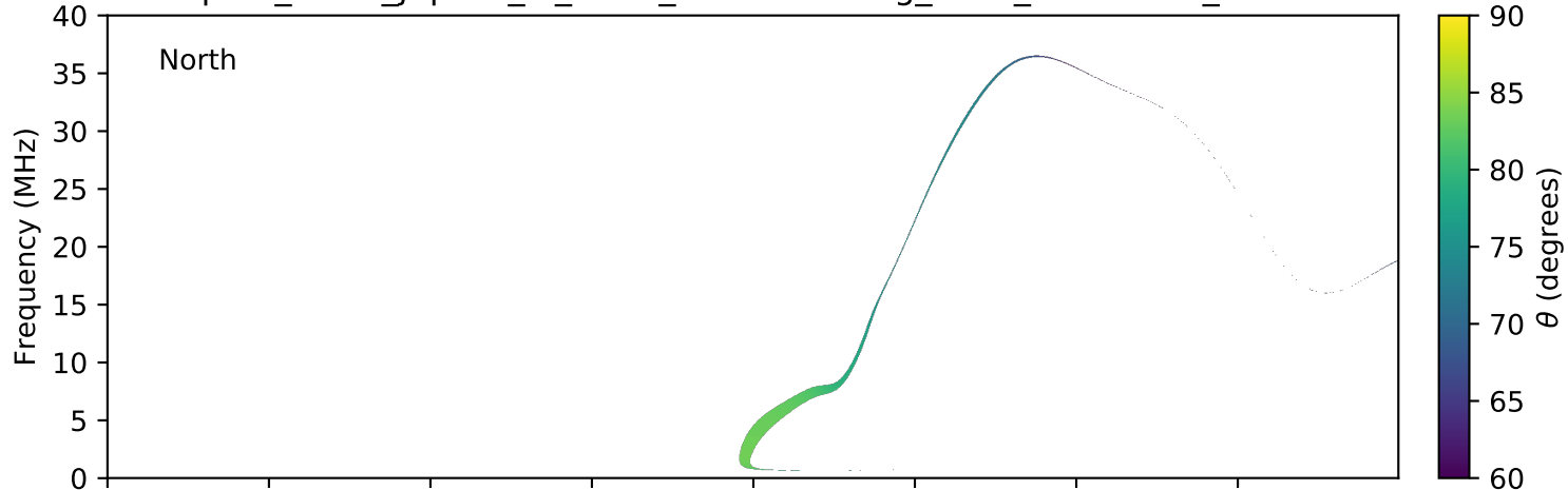
expres_earth_jupiter_io_isaac_lossc-wid1deg_3kev_20100105_v01.cdf
