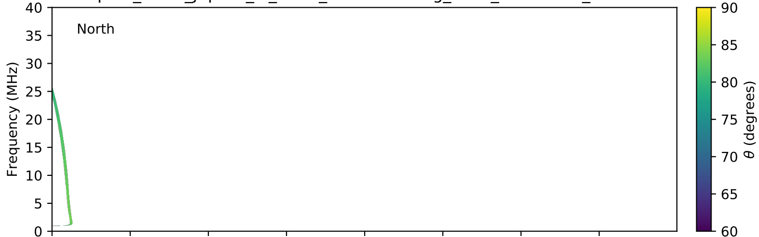
expres_earth_jupiter_io_isaac_lossc-wid1deg_3kev_20100101_v01.cdf
