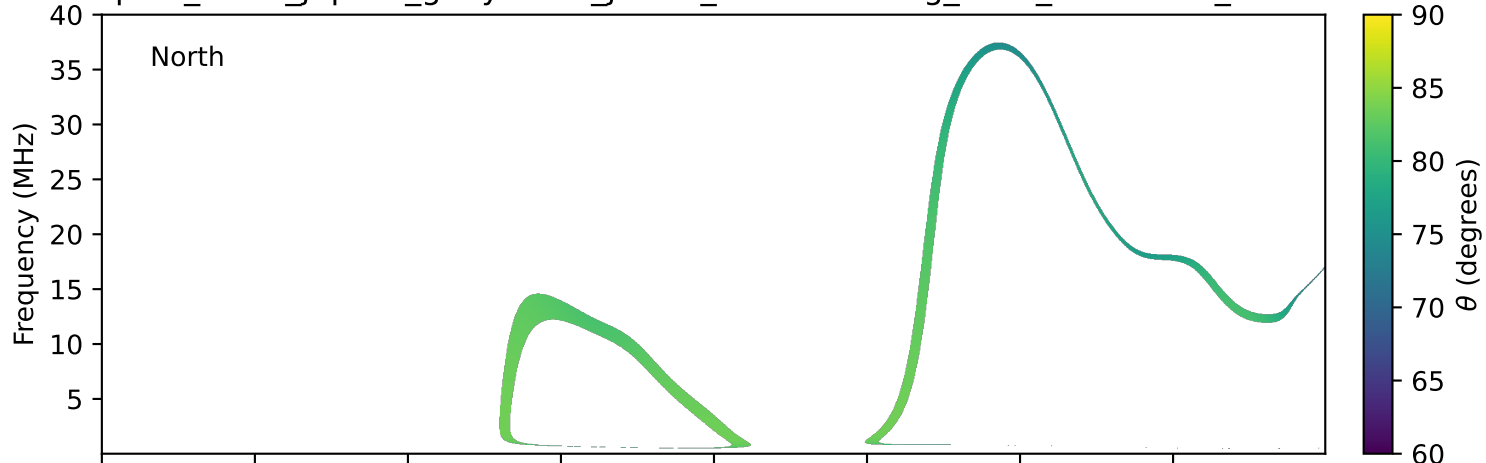
expres_earth_jupiter_ganymede_jrm33_lossc-wid1deg_3kev_20100101_v11.cdf
