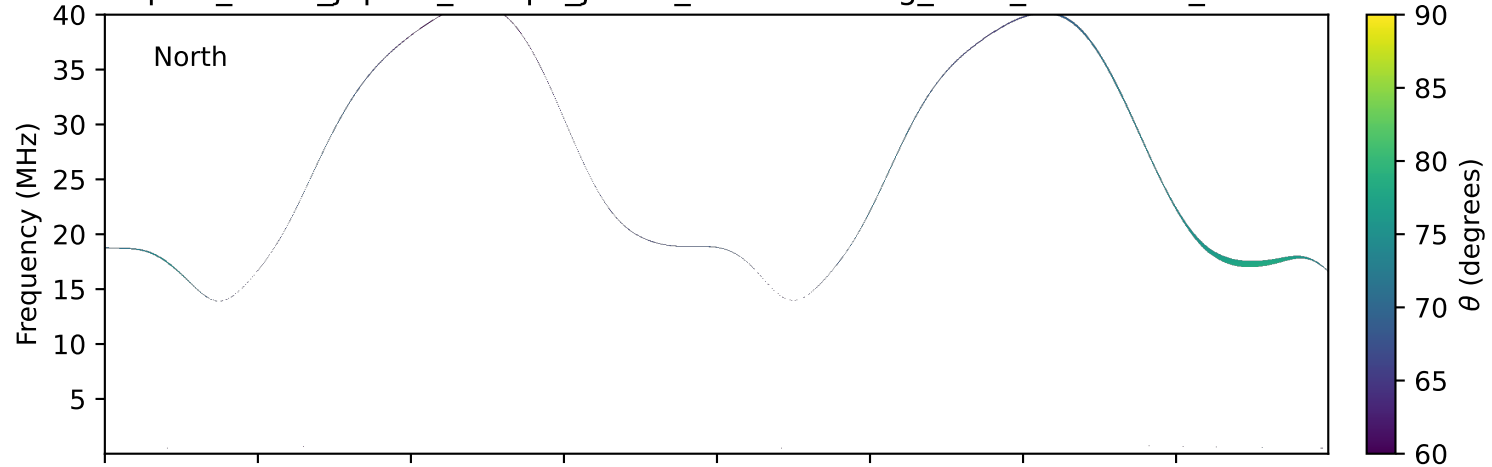
expres_earth_jupiter_europa_jrm33_lossc-wid1deg_3kev_20100123_v11.cdf
