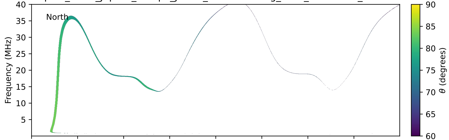
expres_earth_jupiter_europa_jrm33_lossc-wid1deg_3kev_20100119_v11.cdf
