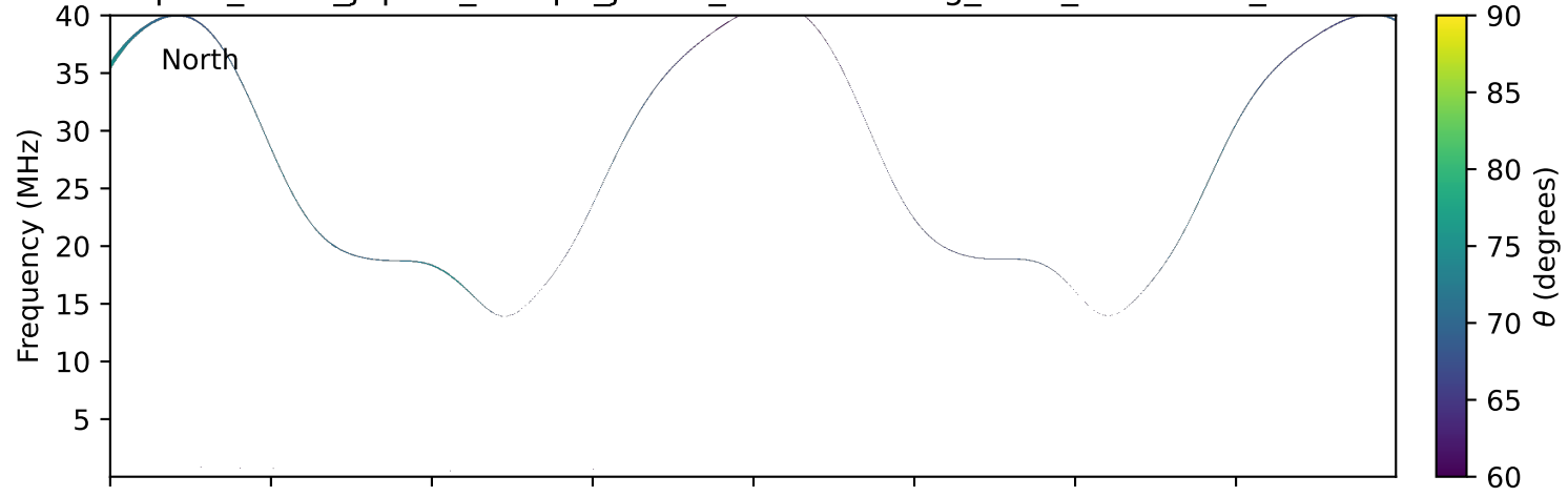
expres_earth_jupiter_europa_jrm33_lossc-wid1deg_3kev_20100105_v11.cdf
