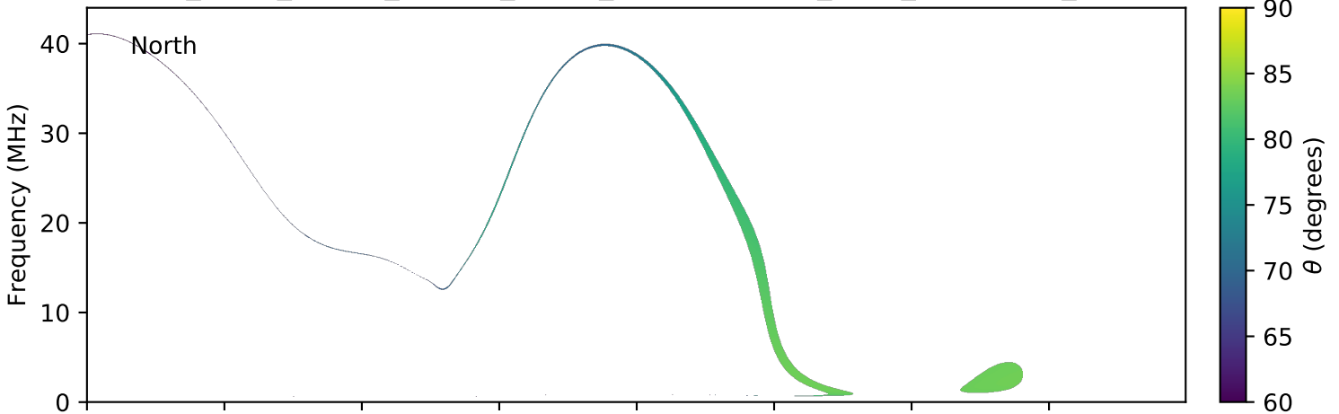
expres_earth_jupiter_europa_jrm09_lossc-wid1deg_3kev_20100127_v01.cdf
