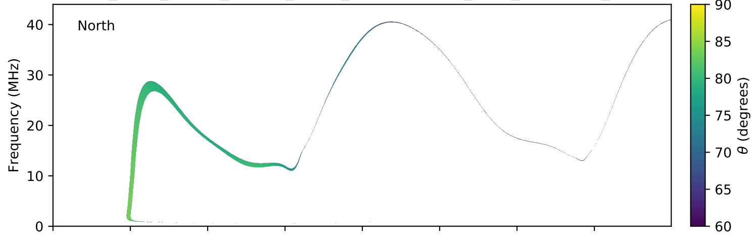
expres_earth_jupiter_europa_jrm09_lossc-wid1deg_3kev_20100126_v01.cdf
