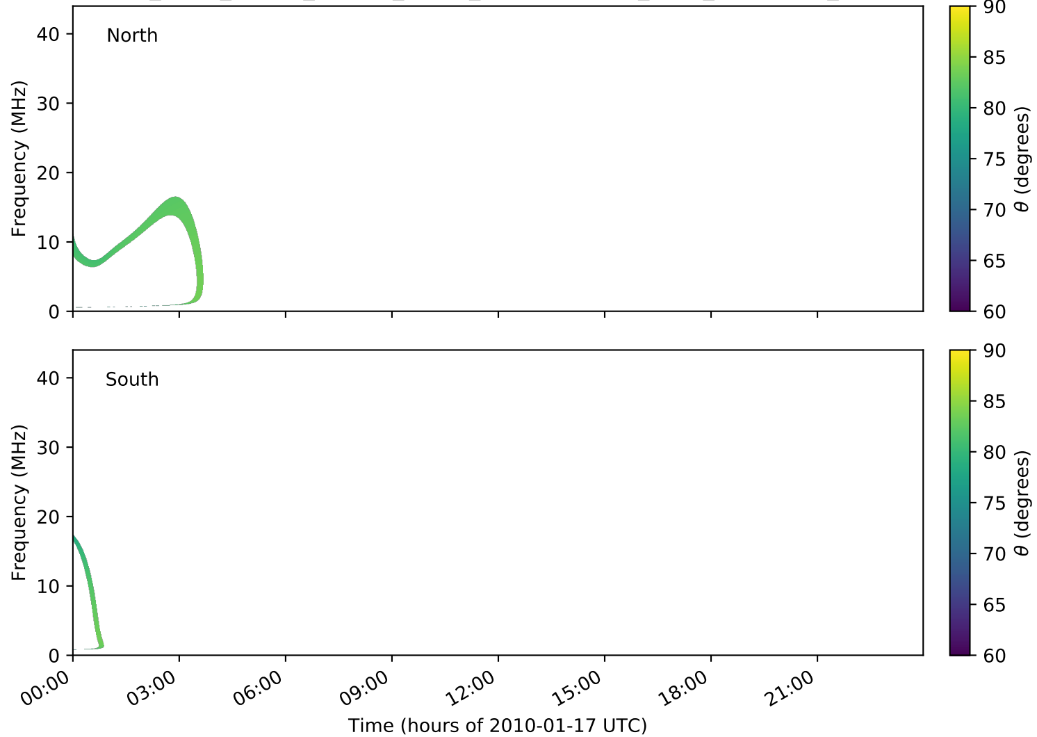
expres_earth_jupiter_europa_jrm09_lossc-wid1deg_3kev_20100117_v01.cdf
