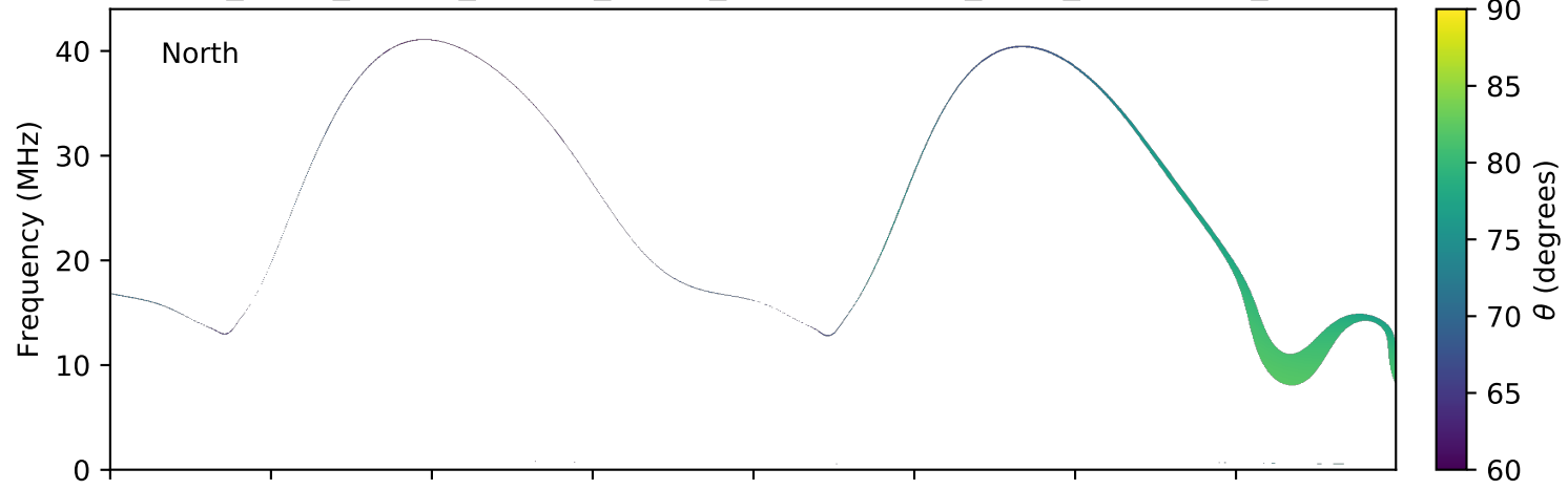
expres_earth_jupiter_europa_jrm09_lossc-wid1deg_3kev_20100116_v01.cdf
