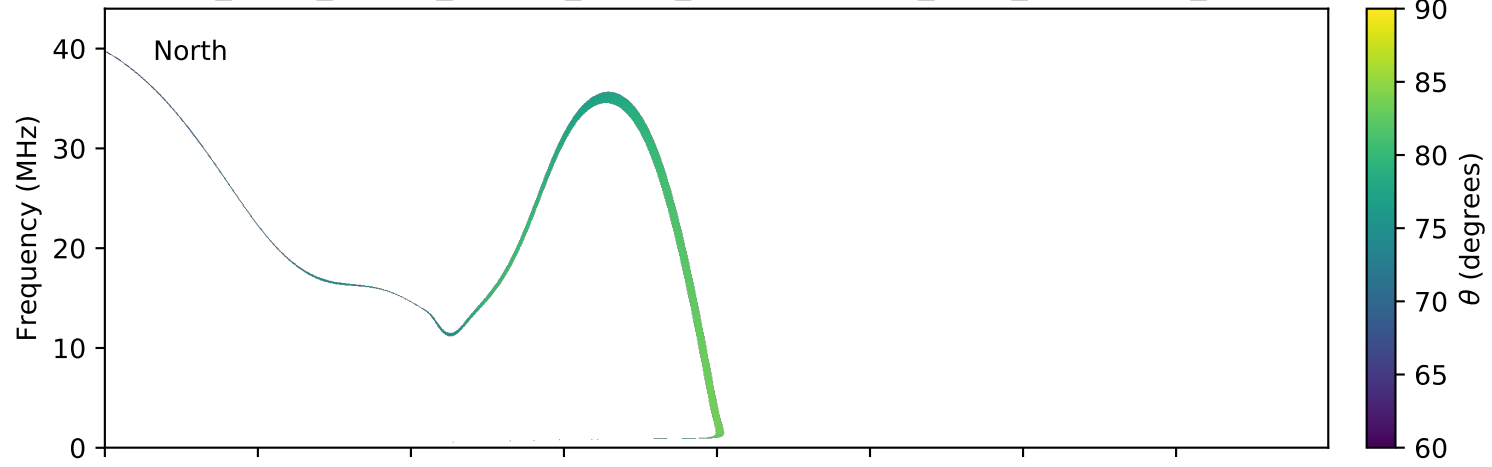
expres_earth_jupiter_europa_jrm09_lossc-wid1deg_3kev_20100113_v01.cdf
