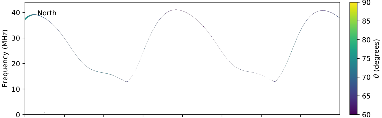
expres_earth_jupiter_europa_jrm09_lossc-wid1deg_3kev_20100105_v01.cdf
