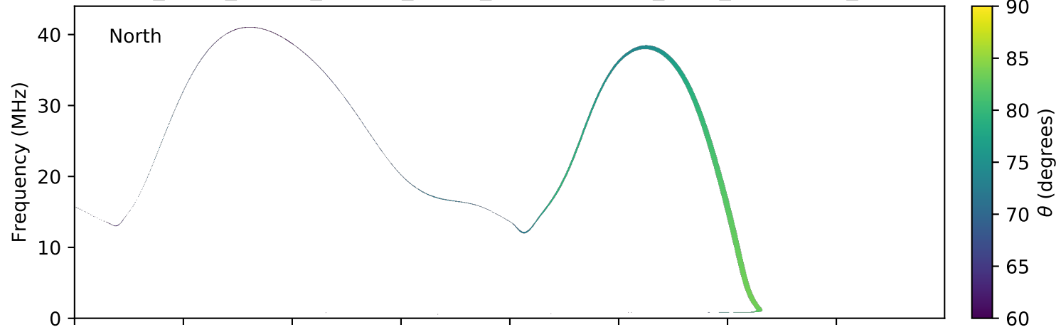
expres_earth_jupiter_europa_jrm09_lossc-wid1deg_3kev_20100102_v01.cdf
