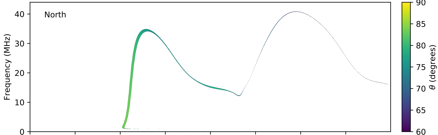
expres_earth_jupiter_europa_jrm09_lossc-wid1deg_3kev_20100101_v01.cdf
