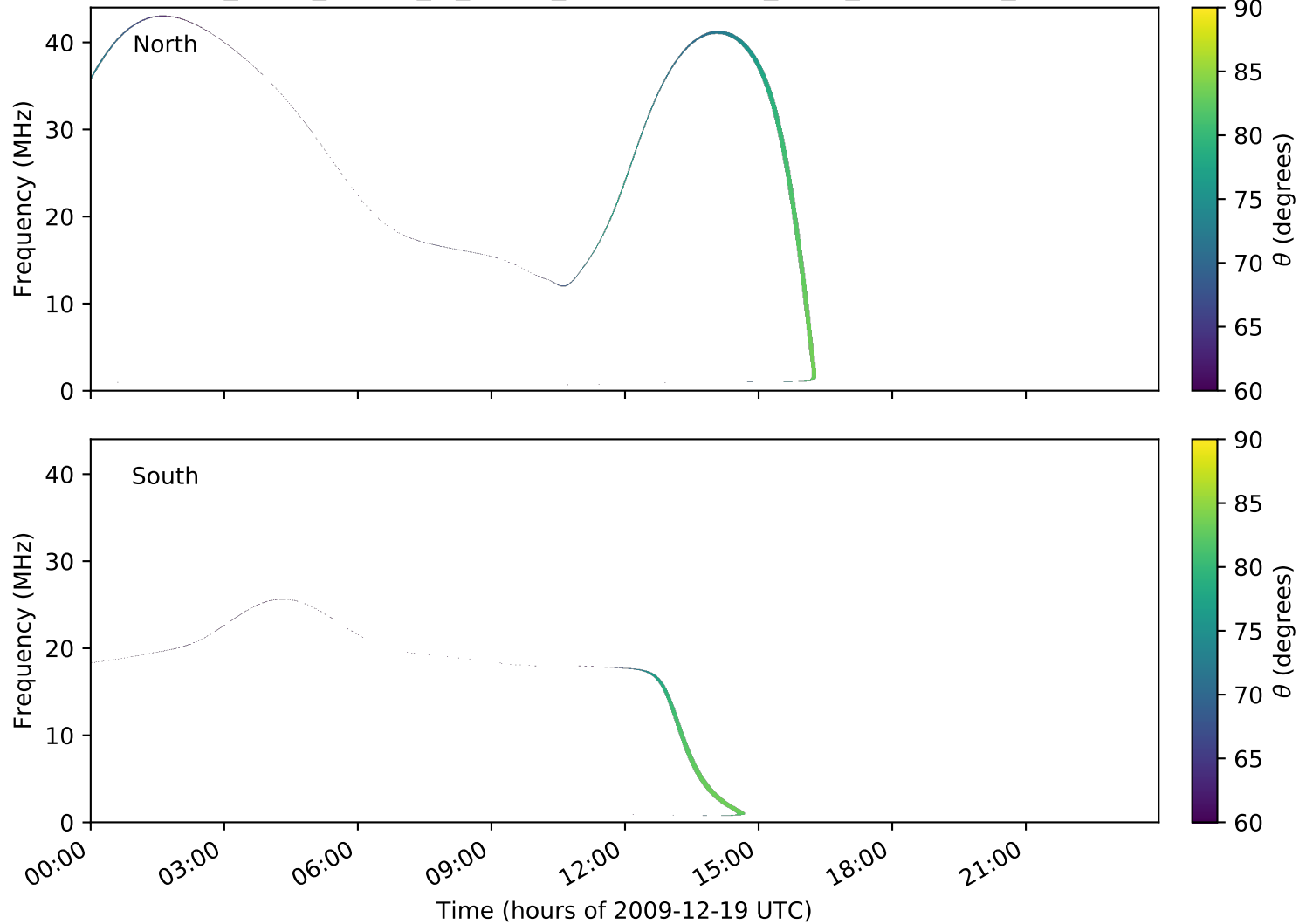
expres_earth_jupiter_io_jrm09_lossc-wid1deg_3kev_20091219_v01.cdf
