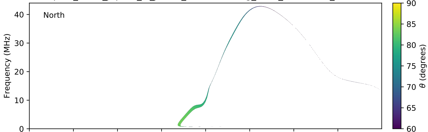
expres_earth_jupiter_io_jrm09_lossc-wid1deg_3kev_20091206_v01.cdf
