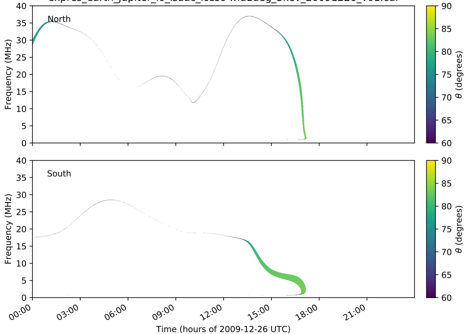
expres_earth_jupiter_io_isaac_lossc-wid1deg_3kev_20091226_v01.cdf
