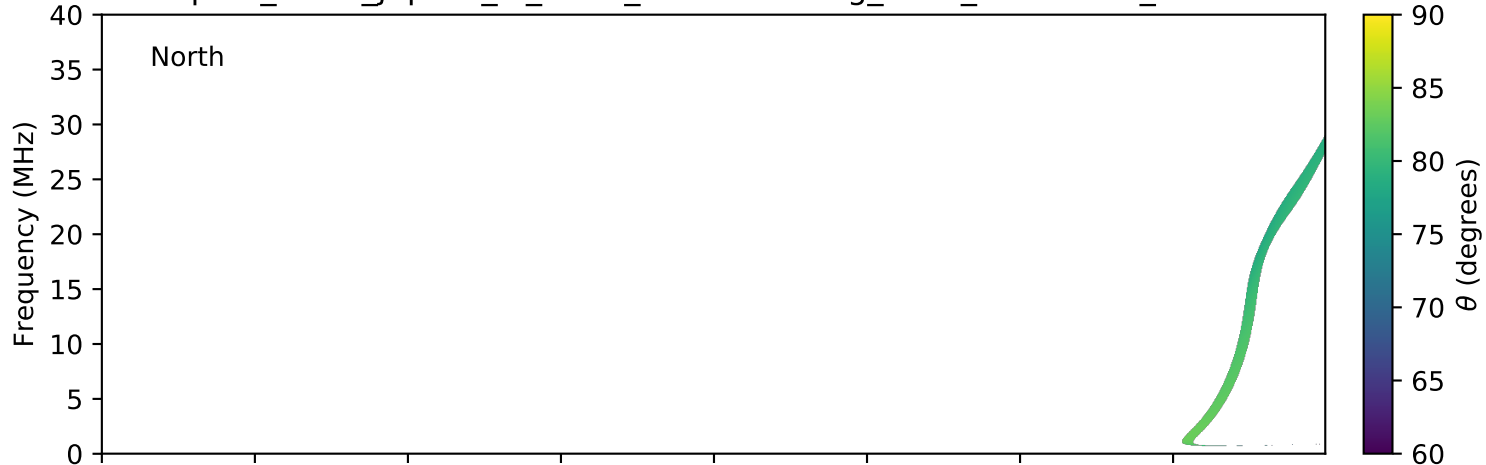
expres_earth_jupiter_io_isaac_lossc-wid1deg_3kev_20091225_v01.cdf
