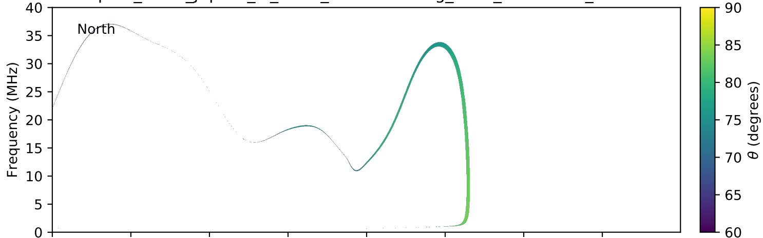
expres_earth_jupiter_io_isaac_lossc-wid1deg_3kev_20091219_v01.cdf
