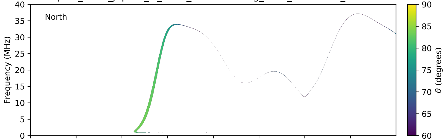
expres_earth_jupiter_io_isaac_lossc-wid1deg_3kev_20091215_v01.cdf
