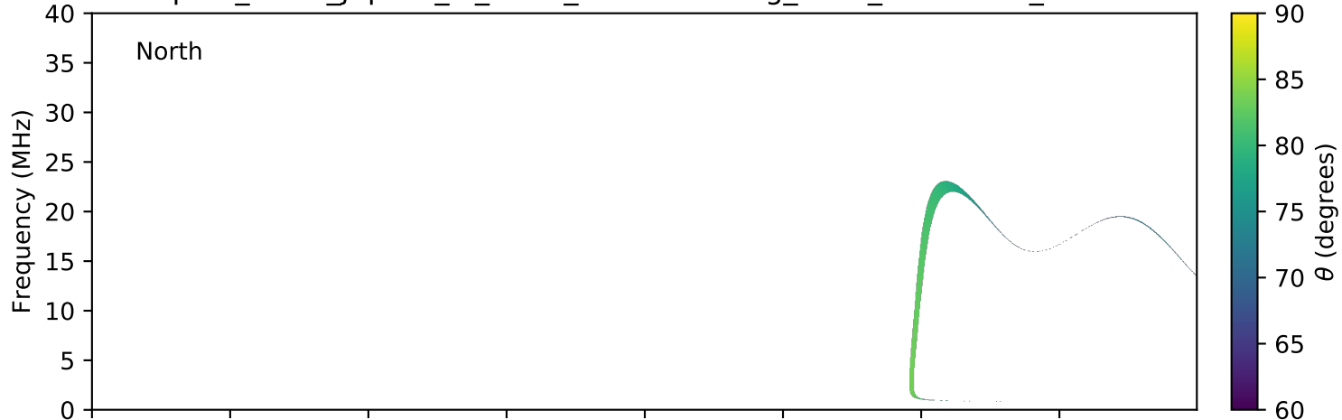
expres_earth_jupiter_io_isaac_lossc-wid1deg_3kev_20091211_v01.cdf
