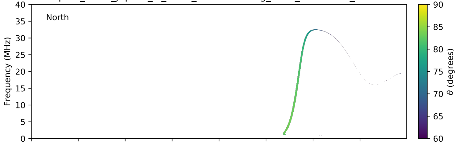
expres_earth_jupiter_io_isaac_lossc-wid1deg_3kev_20091204_v01.cdf
