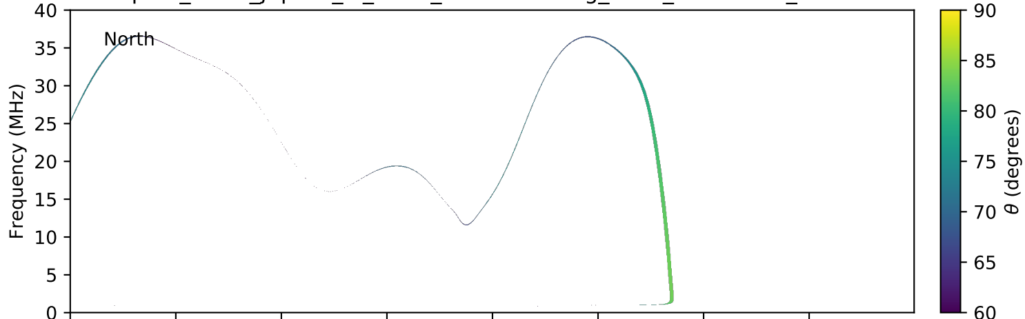
expres_earth_jupiter_io_isaac_lossc-wid1deg_3kev_20091203_v01.cdf
