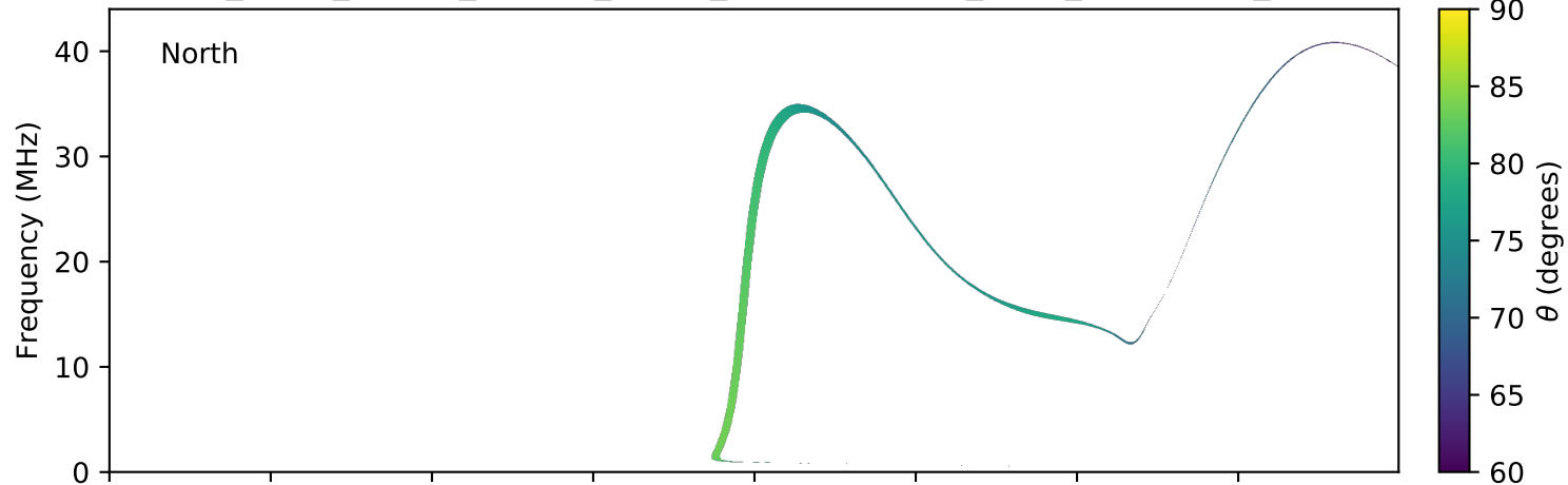
expres_earth_jupiter_europa_jrm09_lossc-wid1deg_3kev_20091214_v01.cdf
