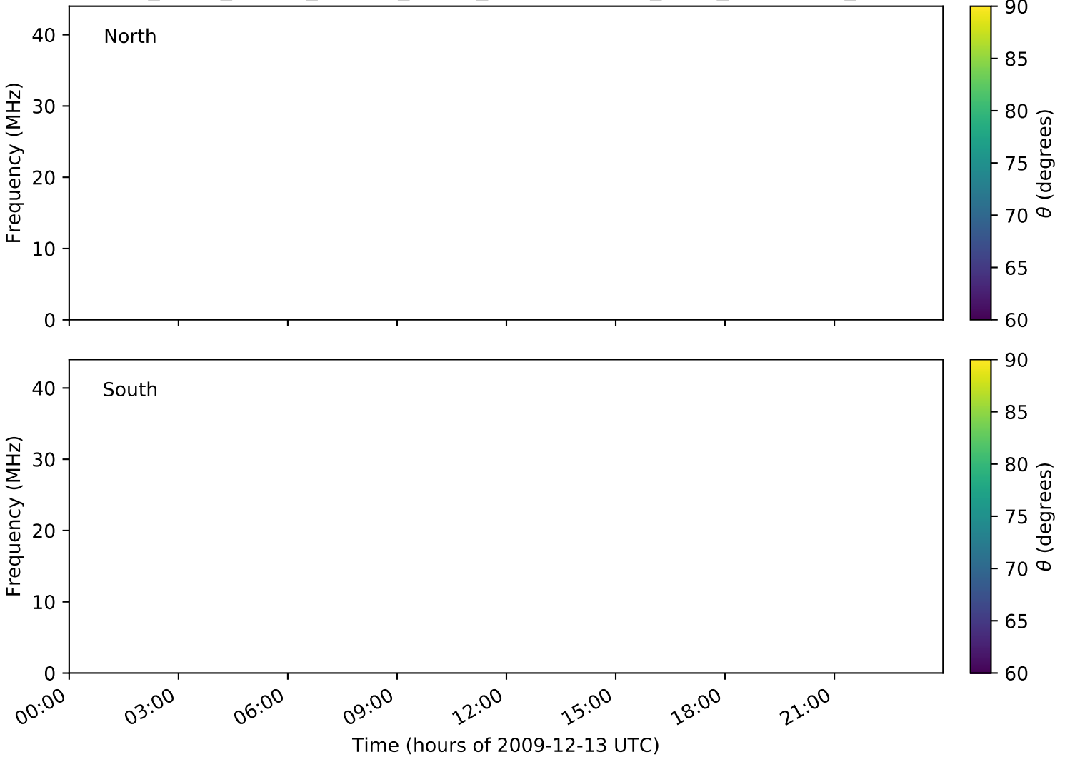
expres_earth_jupiter_europa_jrm09_lossc-wid1deg_3kev_20091213_v01.cdf
