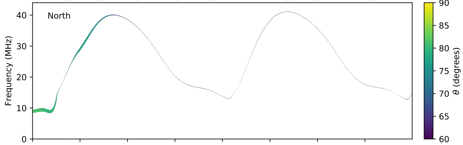
expres_earth_jupiter_europa_jrm09_lossc-wid1deg_3kev_20091211_v01.cdf
