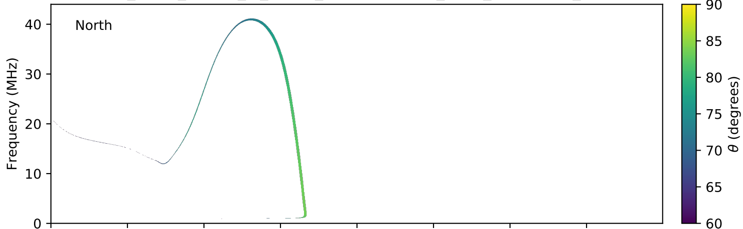
expres_earth_jupiter_io_jrm09_lossc-wid1deg_3kev_20091105_v01.cdf
