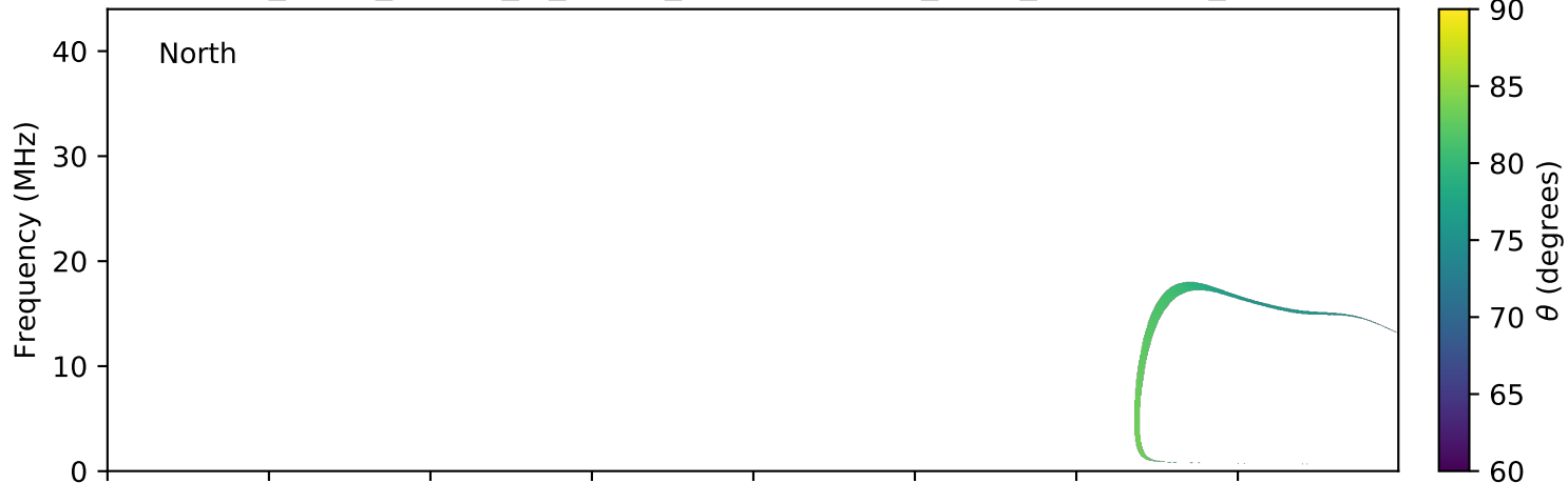
expres_earth_jupiter_io_jrm09_lossc-wid1deg_3kev_20091102_v01.cdf
