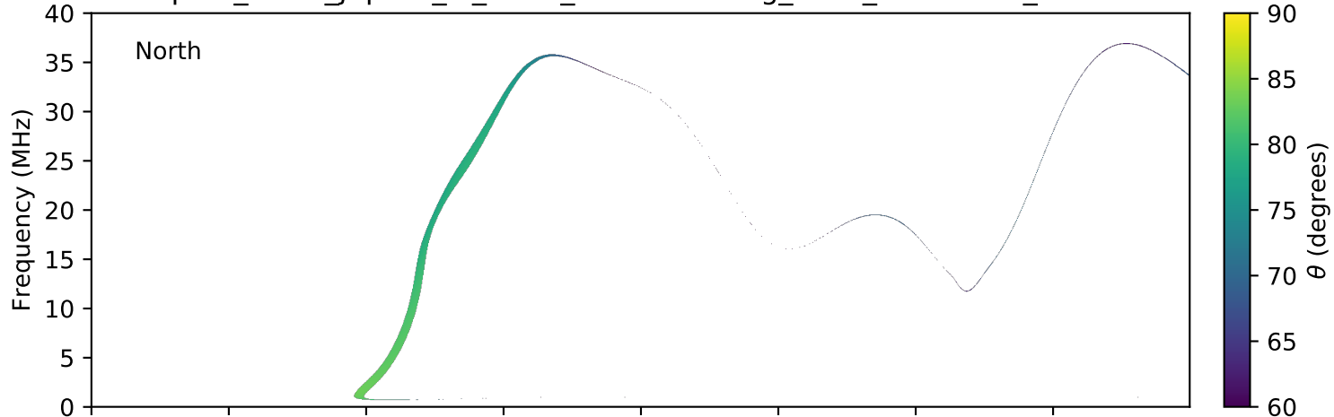
expres_earth_jupiter_io_isaac_lossc-wid1deg_3kev_20091122_v01.cdf
