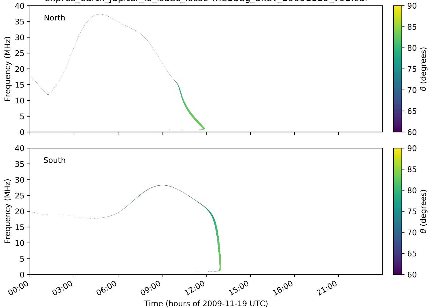
expres_earth_jupiter_io_isaac_lossc-wid1deg_3kev_20091119_v01.cdf
