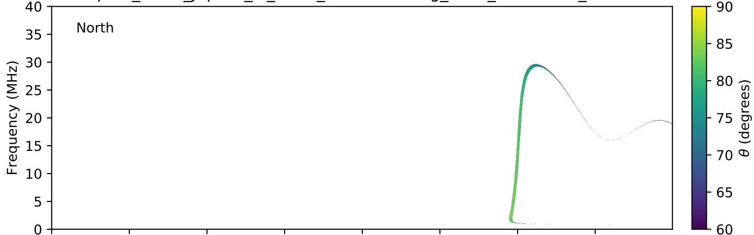
expres_earth_jupiter_io_isaac_lossc-wid1deg_3kev_20091118_v01.cdf
