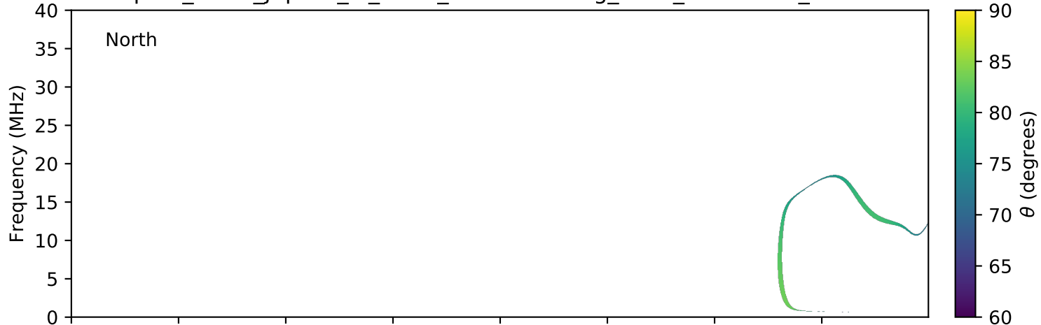
expres_earth_jupiter_io_isaac_lossc-wid1deg_3kev_20091109_v01.cdf
