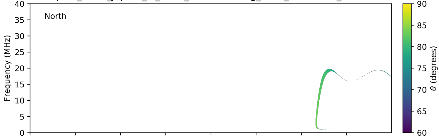
expres_earth_jupiter_io_isaac_lossc-wid1deg_3kev_20091102_v01.cdf
