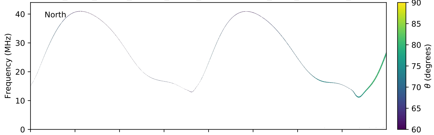
expres_earth_jupiter_europa_jrm09_lossc-wid1deg_3kev_20091120_v01.cdf
