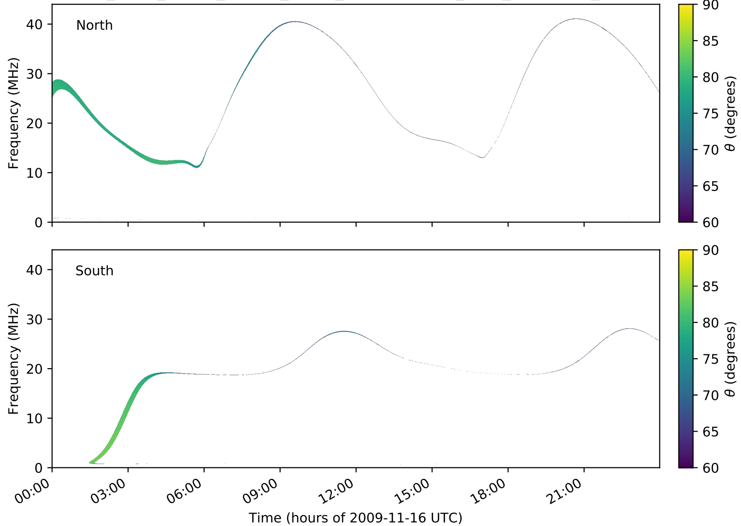
expres_earth_jupiter_europa_jrm09_lossc-wid1deg_3kev_20091116_v01.cdf
