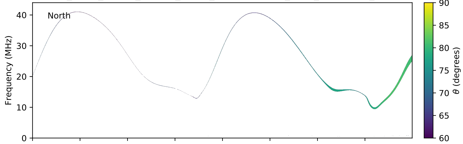
expres_earth_jupiter_europa_jrm09_lossc-wid1deg_3kev_20091113_v01.cdf
