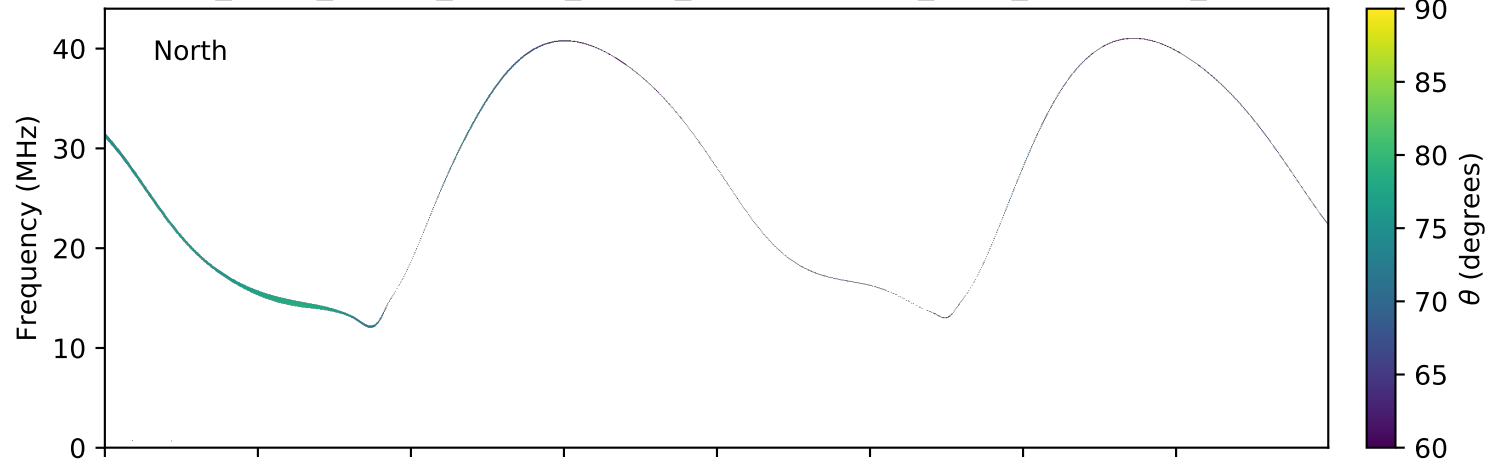
expres_earth_jupiter_europa_jrm09_lossc-wid1deg_3kev_20091109_v01.cdf
